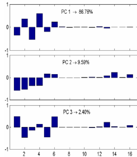
Figure 2. The first three angular momentum primitives in the sagittal plane and their respective data explained. The abscissa numbers and human model links are paired in the following order: left foot (1), right foot (2), left shin (3), right shin (4), left thigh (5), right thigh (6), left hand (7), right hand (8), left forearm (9), right forearm (10), left upper arm (11), right upper arm (12), abdomen and pelvis (13), thorax (14), neck (15) and head (16).
