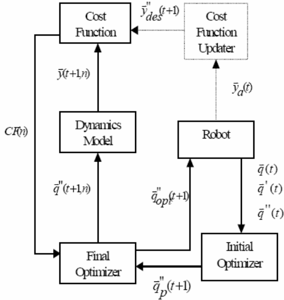
Figure 4. Block diagram of controller. The vectors \bar{q}(t) , \bar{q}'(t) and \bar{q}''(t) denote the position, velocity and acceleration of the robot's joints.
