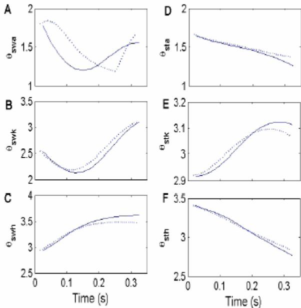
Figure 6. Simulation joint angles (solid lines) are compared with joint angles from biological gait data (dotted line). A) Swing ankle. B) Swing knee. C) Swing hip. D) Stance ankle. E) Stance knee. F) Stance hip.
