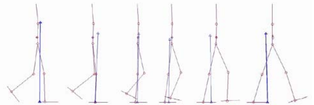
Figure 5. Six consecutive poses from the simulation of the sagittal model in the single support phase. The target CM is represented with a cross and the actual simulation's CM is denoted with a diamond. The ground reaction force vector is represented with an arrow and it originates at the FRI point moving beneath the stance foot. The force magnitude is represented so that 1 N corresponds to 2 mm of the actual humanoid model's dimensions. Height of the CM is approximately 1 m.
